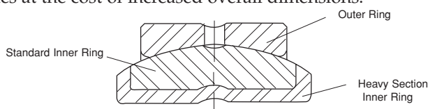
Figure 5: Standard vs. Heavy Section Inner Ring
