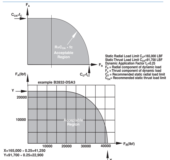
Fig. 15: Angular Contact Bearings, Double Acting
