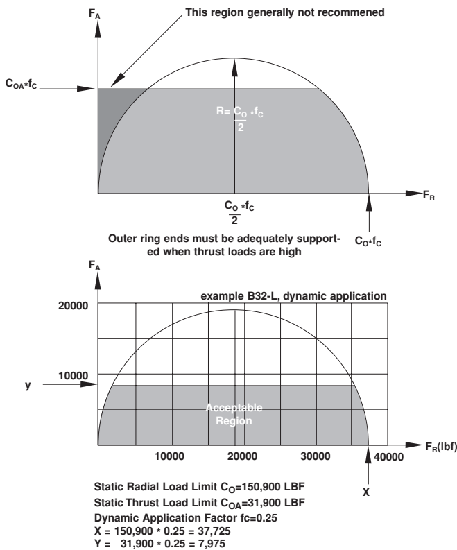
Figure 13: Radial Bearings
