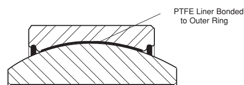
Figure 8: Maintenance-Free Bearings
