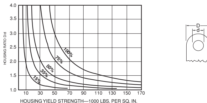
Figure 17: Influence of Housing Design on Bearing Capacity
