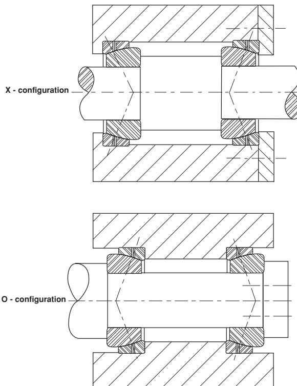
Figure 10: Bearing Arrangement
