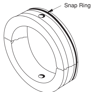
Figure 2: Double Fractured Outer Ring
