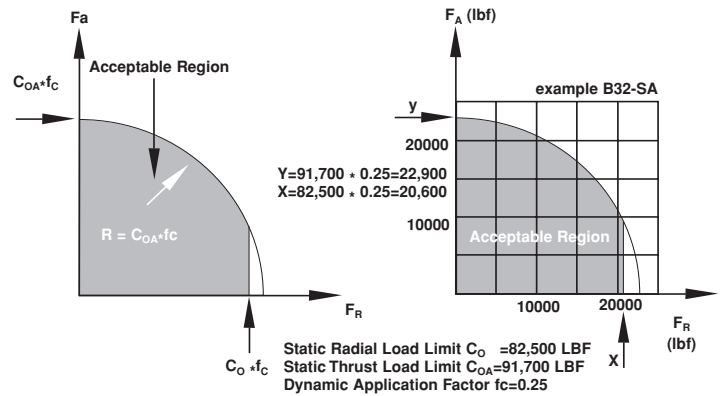
Figure 14: Angular Contact Bearings, Single Acting
