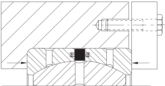
Figure 12: ShimPack® Compression Force=F c
